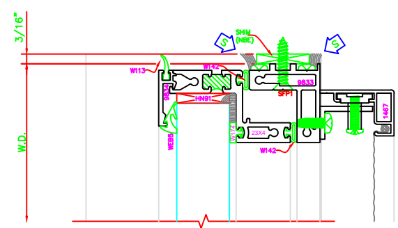
102 HEAD WW410
