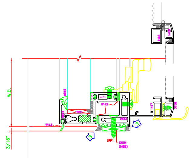
202 SILL WW410
